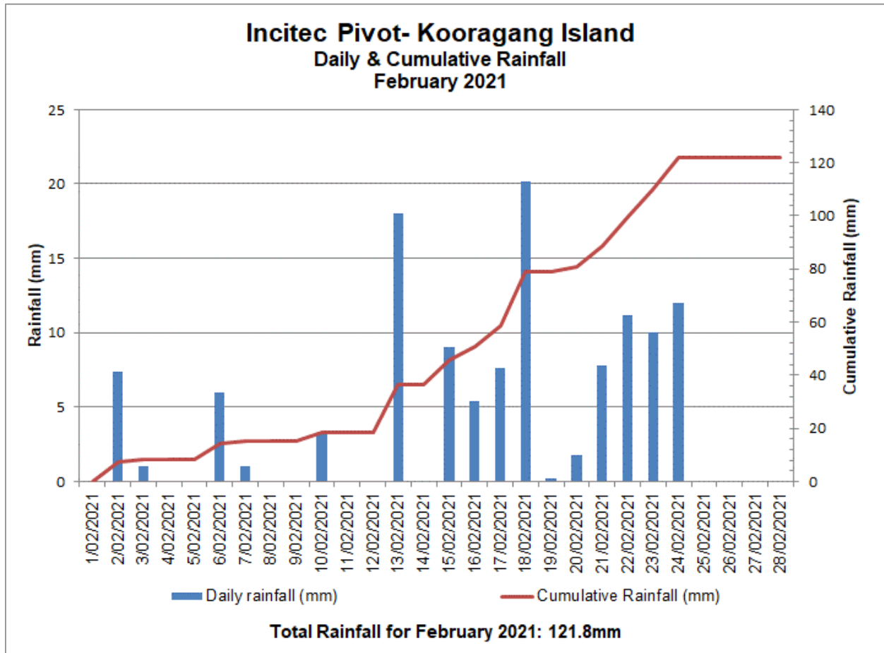
Figure 1 February 2021 Rainfall Summary
