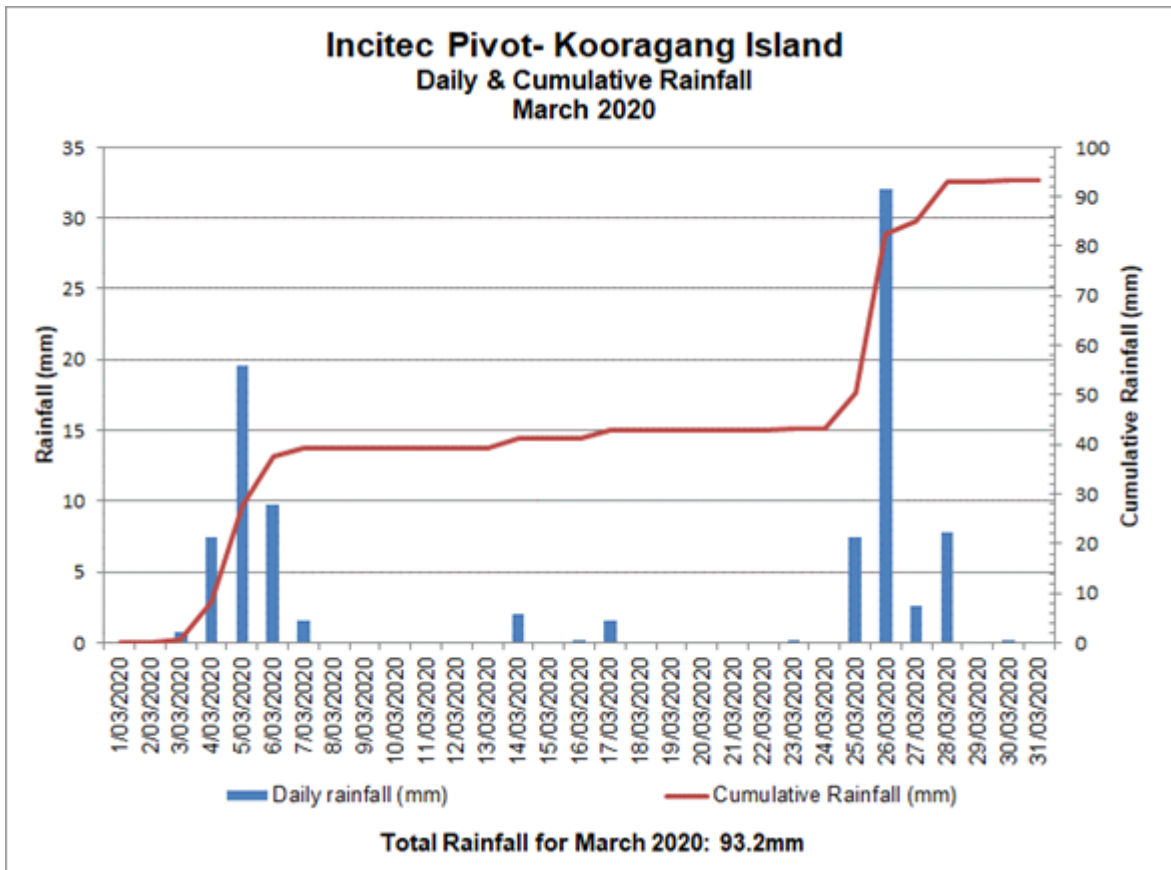
Figure 1 March 2020 Rainfall Summary
